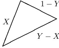
Figure 6.3.2: Random Triangle
