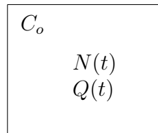
Figure 1: One-Compartment Model
