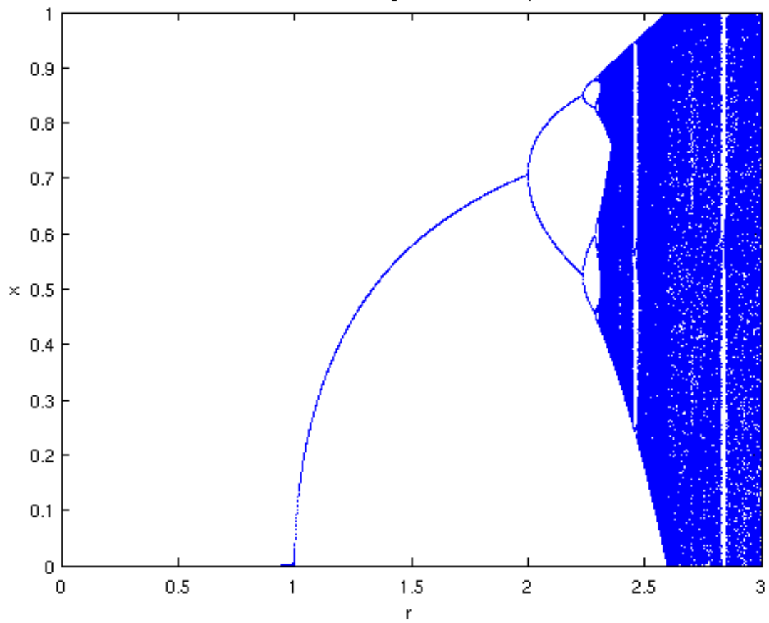
Bifurcation Diagram for Cubic Map
