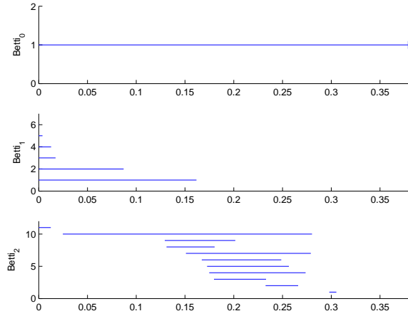
Figure 13: PLEX results for \mathcal{A}_{0,50}
