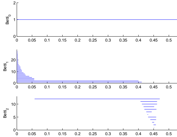
Figure 12: PLEX results for \mathcal{K}
