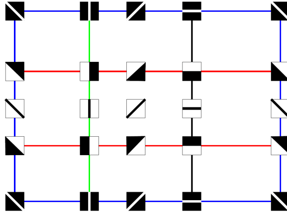
Figure 6: 3 by 3 patches parametrized by the Klein bottle
