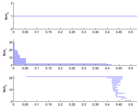
Figure 14: PLEX results for \mathcal{K}_2
