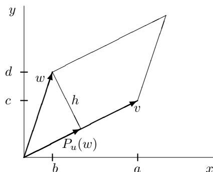
Figure 4.6.12: Parallelogram P(v, w) in the xy -plane
