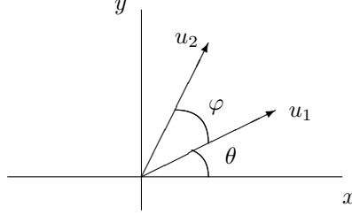
Figure 4.5.10: Angle between u_1 and u_2
