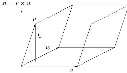
Figure 4.6.14: Volume of Parallelepiped
