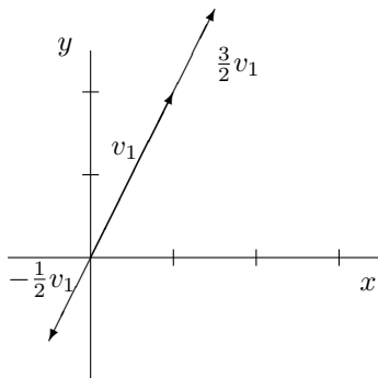
Figure 2.2.5: Scalar Multiplication
