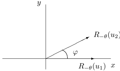
Figure 4.5.11: Angle between R_{-\theta}(u_1) and R_{-\theta}(u_2)
