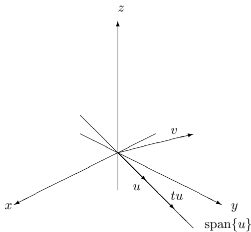
Figure 4.2.4: Orthogonal Projection
