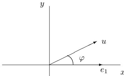
Figure 4.5.9: Angle between u and e_1
