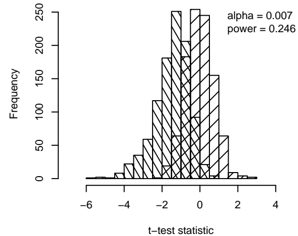
outlier data / t-test
