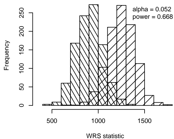
double exponential data / WRS test
