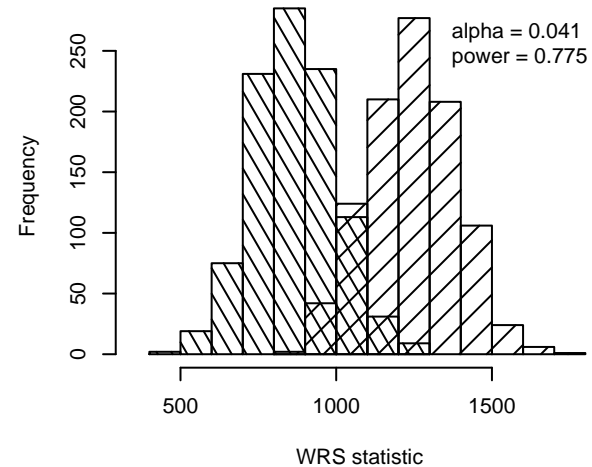
outlier data / WRS test
