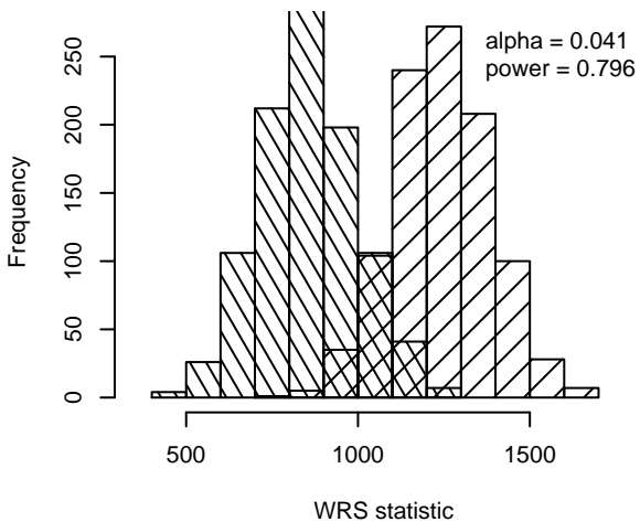
normal data / WRS test
